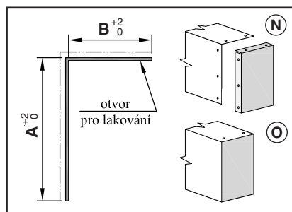
KP 1b L = A + B
