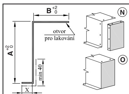
KP 1c L = X + A + B
