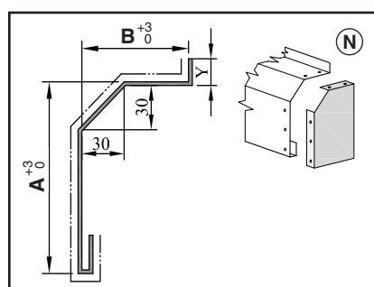
KP 2d L = A + B + Y
